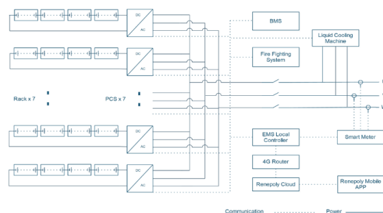
Renepoly ES4598 System Configuration
